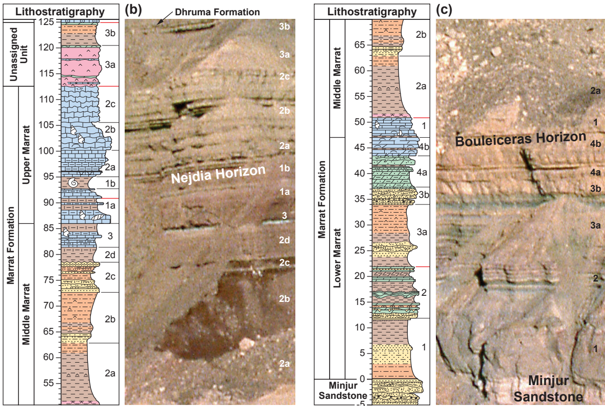
Photo 1: (a) Panoramic photo of the Dhibi Escarpment taken from a helicopter showing the upper Minjur Sandstone, Marrat Formation and Lower Dhurma. The Middle Dhurma crops out in the overlying plateau and hills, and farther west the Upper Dhurma and Tuwaiq Mountain Limestone form the Tuwaiq Mountain Escarpment. The Dhibi Escarpment is most prominent in the Darma', Wadi ar Rayn and Wadi al Mulayh Quadrangles; south of 21°45'N in the Sulayyimiya Quadrangle it merges with the Tuwaiq Mountain Escarpment (Figure 2). (b and c) Comparison between the reference section measured at Khashm adh Dhibi locality and two extracts from Photo (a).
